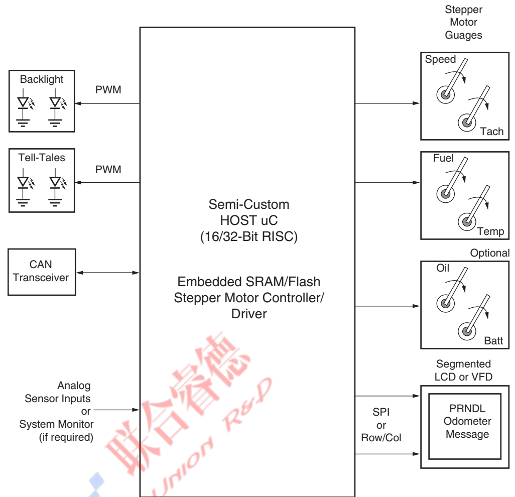
Figure 3: Traditional Cluster Architecture
